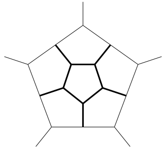
Pentacon P
