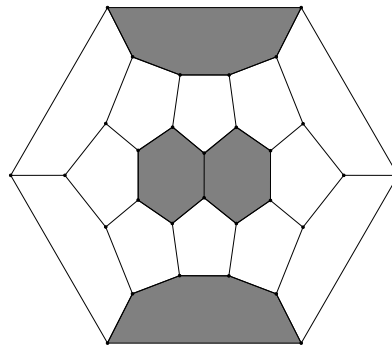
30, C_{2v}
