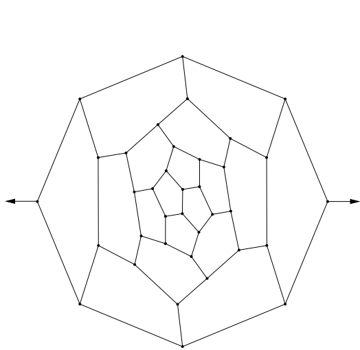
36, D_2
