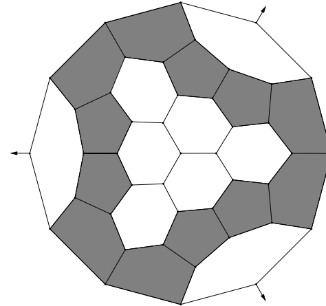
44, D_{3d}
