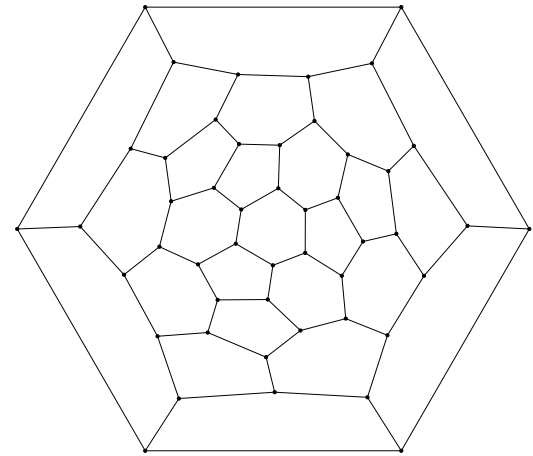
48, D_3
