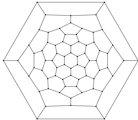
72, D_{2d}
