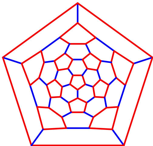
C_{60}(I_h) : (1, 1)- dodecahedron
