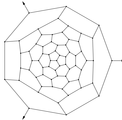
68, D_{3d}
