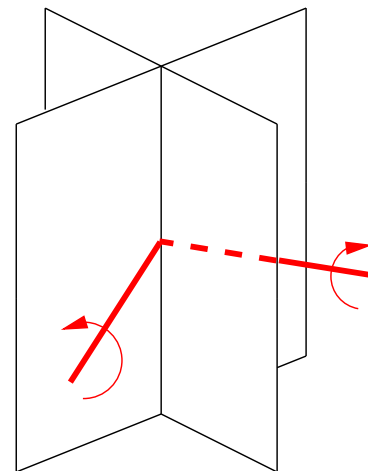
D_{2d}
