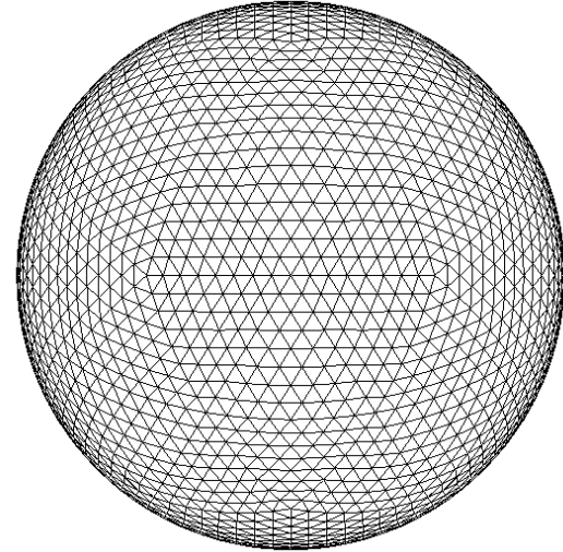
Dual 4-cham. dodecahedron C_{5120}^*, (a, b) = (2^4 = 16, 0), I_h
