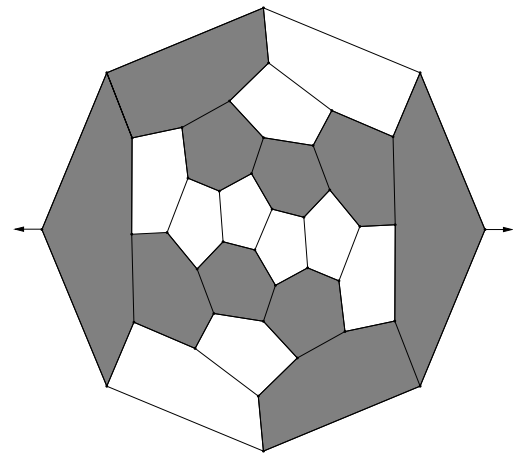
40, D_2
