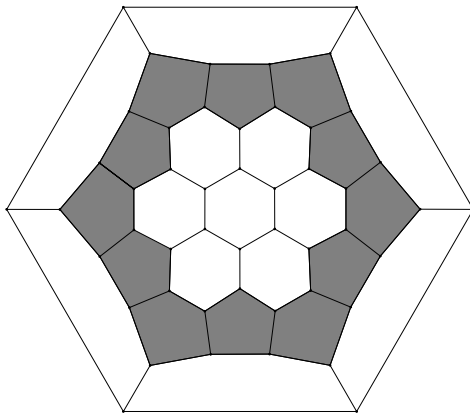
48, D_{6d}
