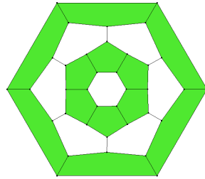
36, D_{6h}
