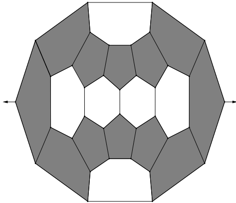
36, D_{2d}
