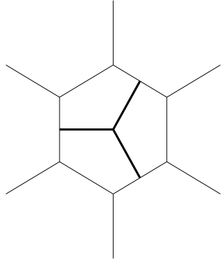
Triacon T_1
