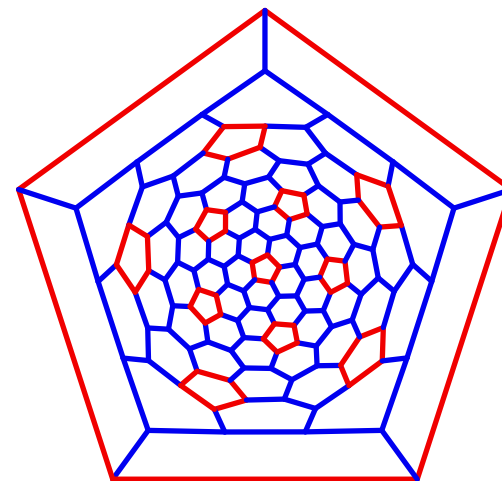
C_{140}(I) : (2, 1)- dodecahedron
