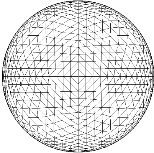
Dual 4-chamfered cube (a, b) = (2^4 = 16, 0), O_h
