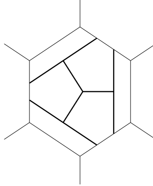
Triacon T_2
