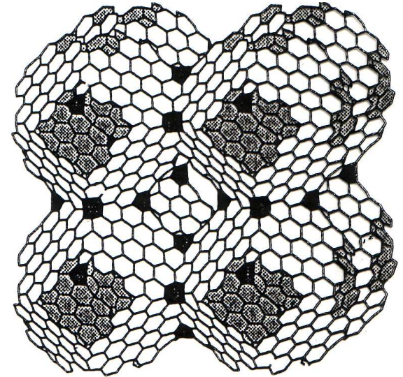
(1, 2)
