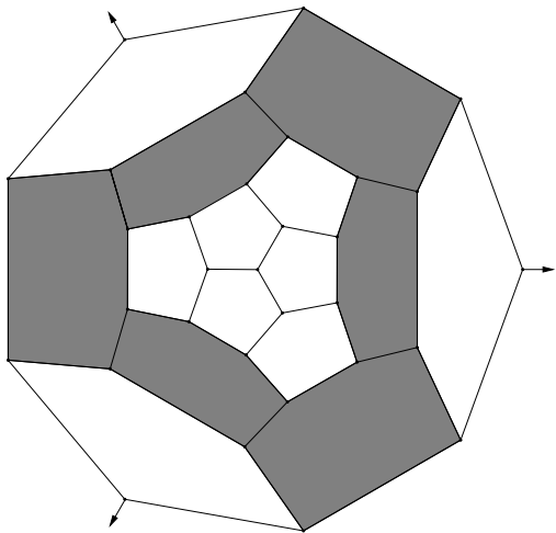
32, D_{3d}
