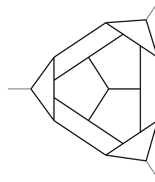
Triacon T_3
