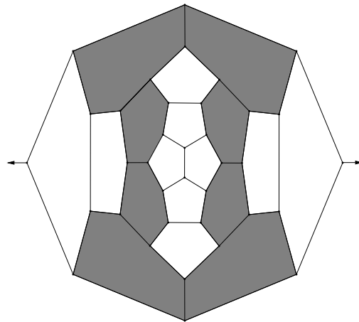
36, D_{2d}
