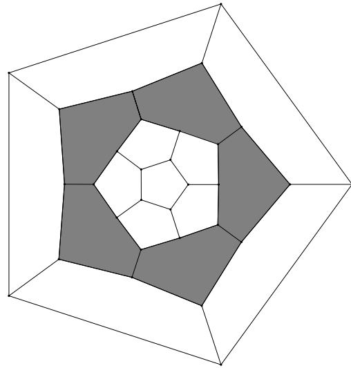
30, D_{5h}
