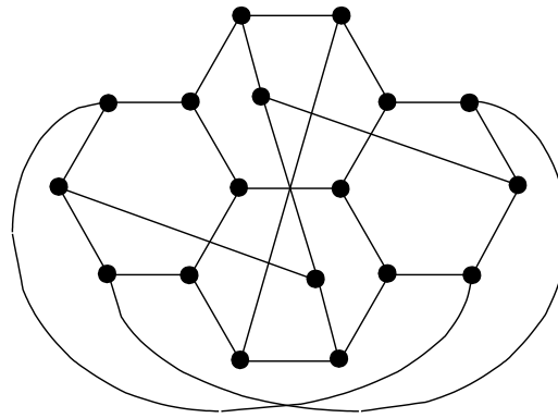
Klein bottle fullerene
