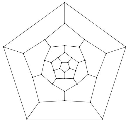
40, D_{5d}
