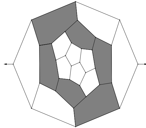
32, D_2
