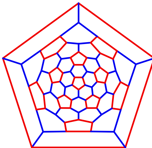
C_{80}(I_h) : (2, 0)- dodecahedron
