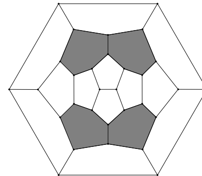
30, C_{2v}
