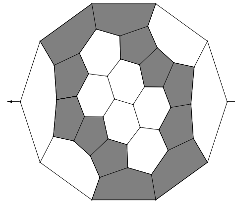
44, D_2
