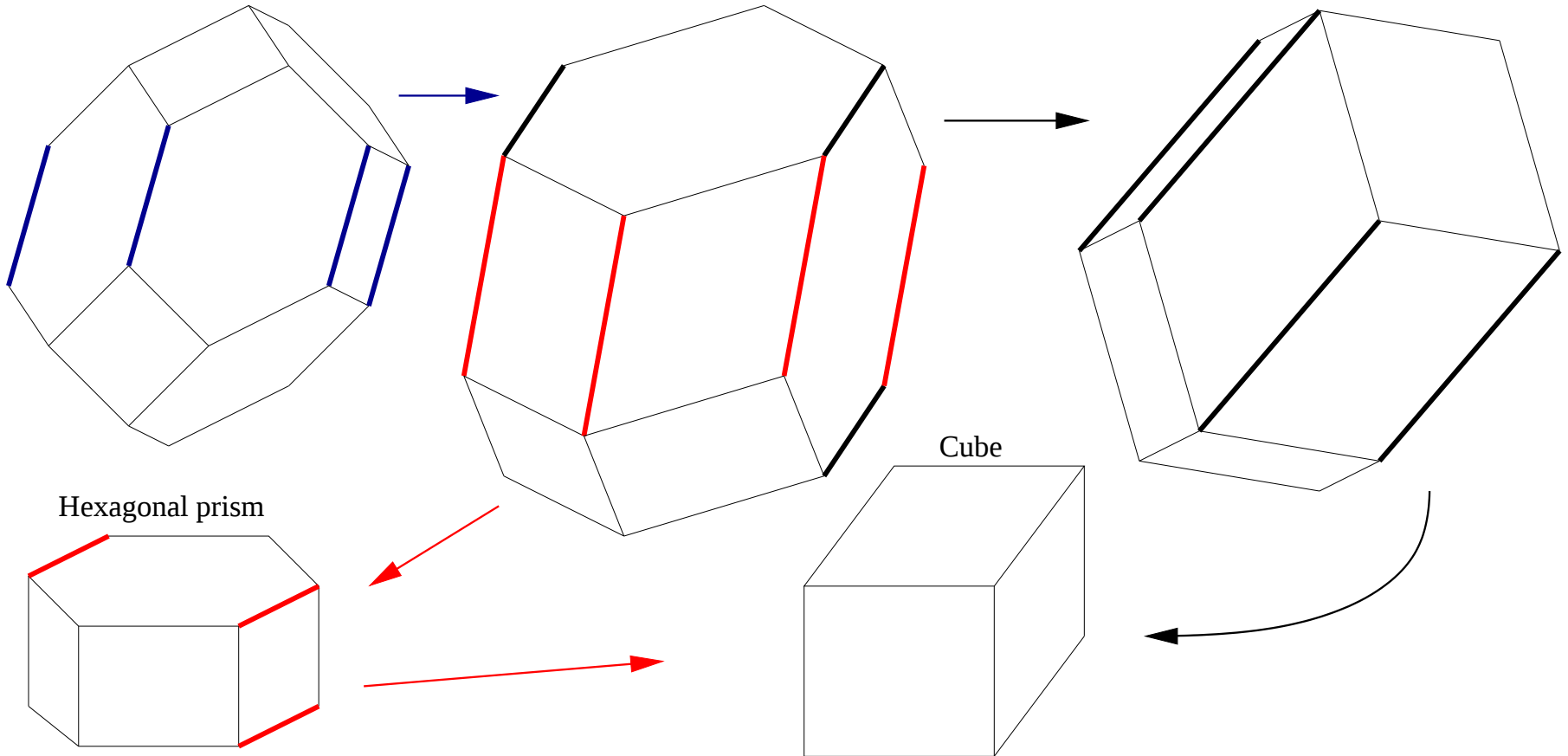
Truncated octahedron
