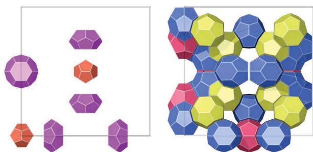
Figure 2 The inflation on the A_{15} structure: the shrunk cells of A_{15} and the generated F_{28} .
