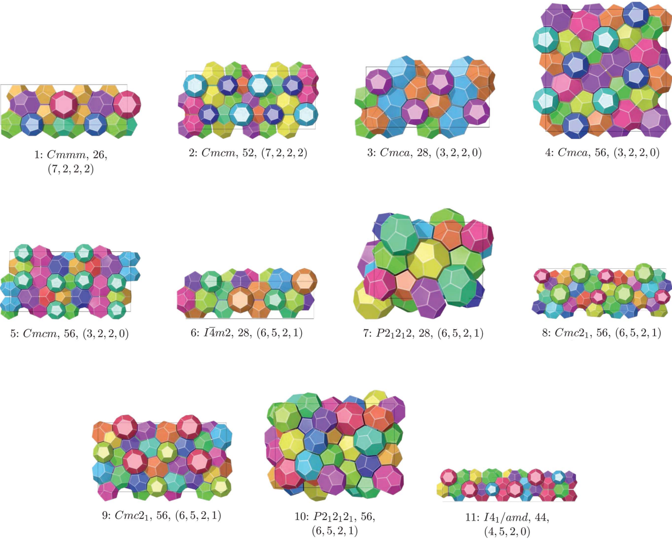
Figure 6 New space fullerenes with known fraction.
