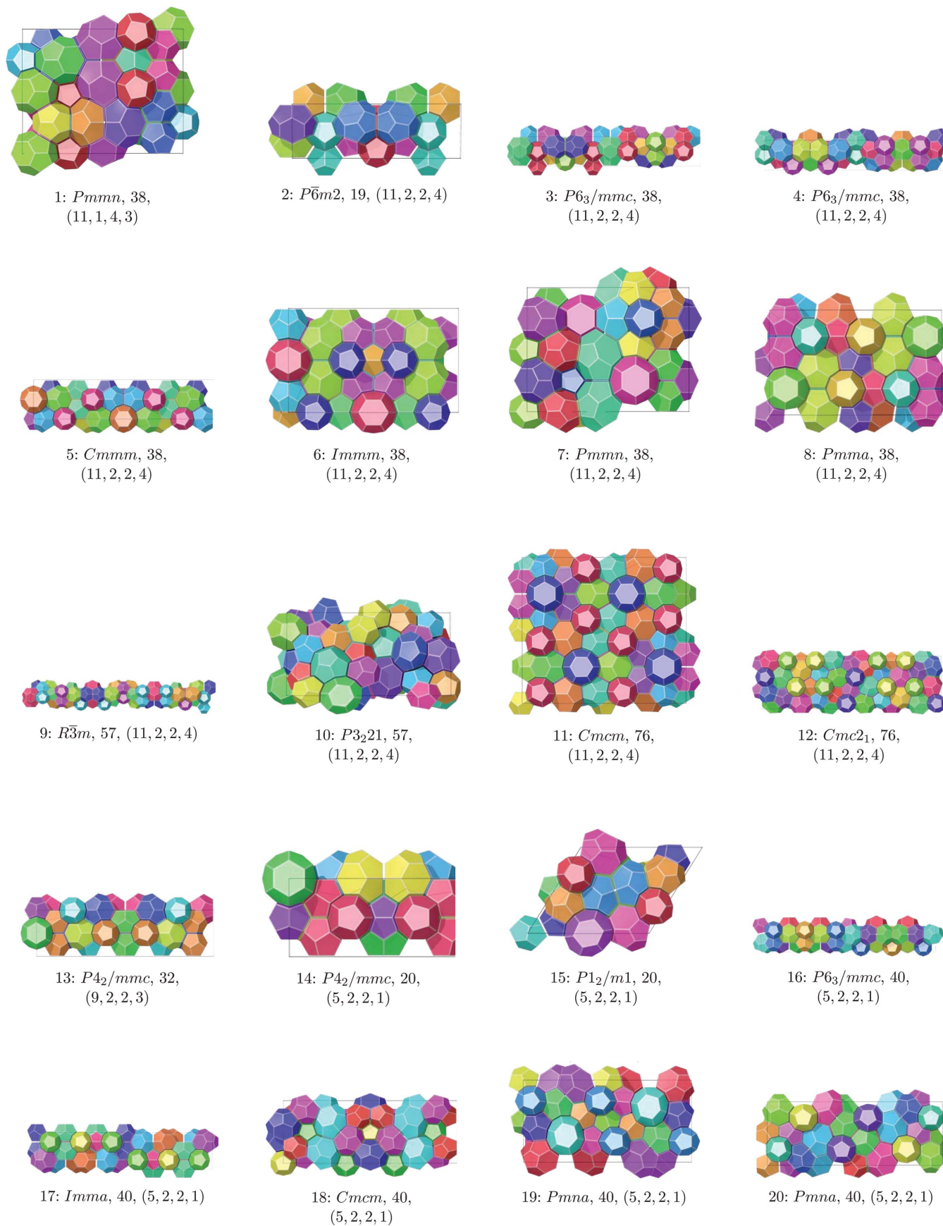
Figure 7 Other new space fullerenes.
